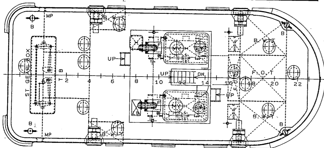
UP DECK PLAN
