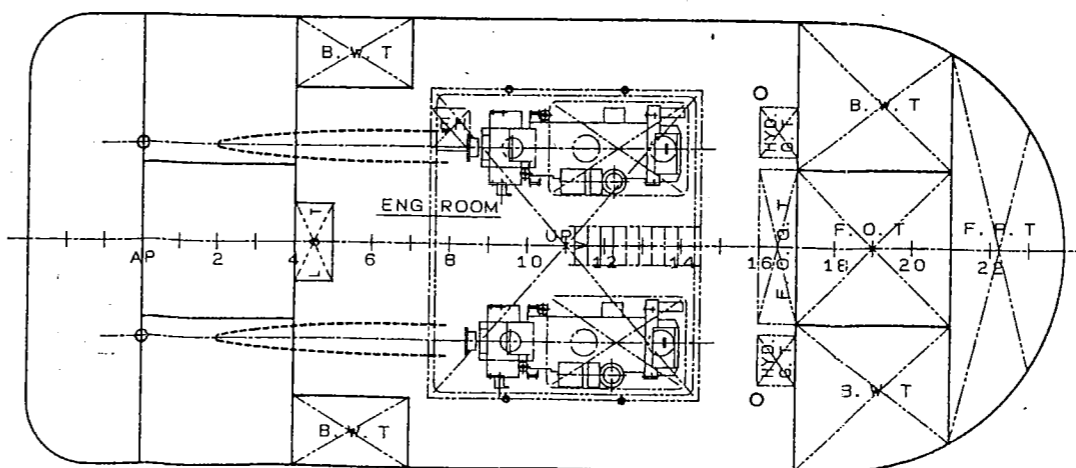
BOTTOM PLAN
